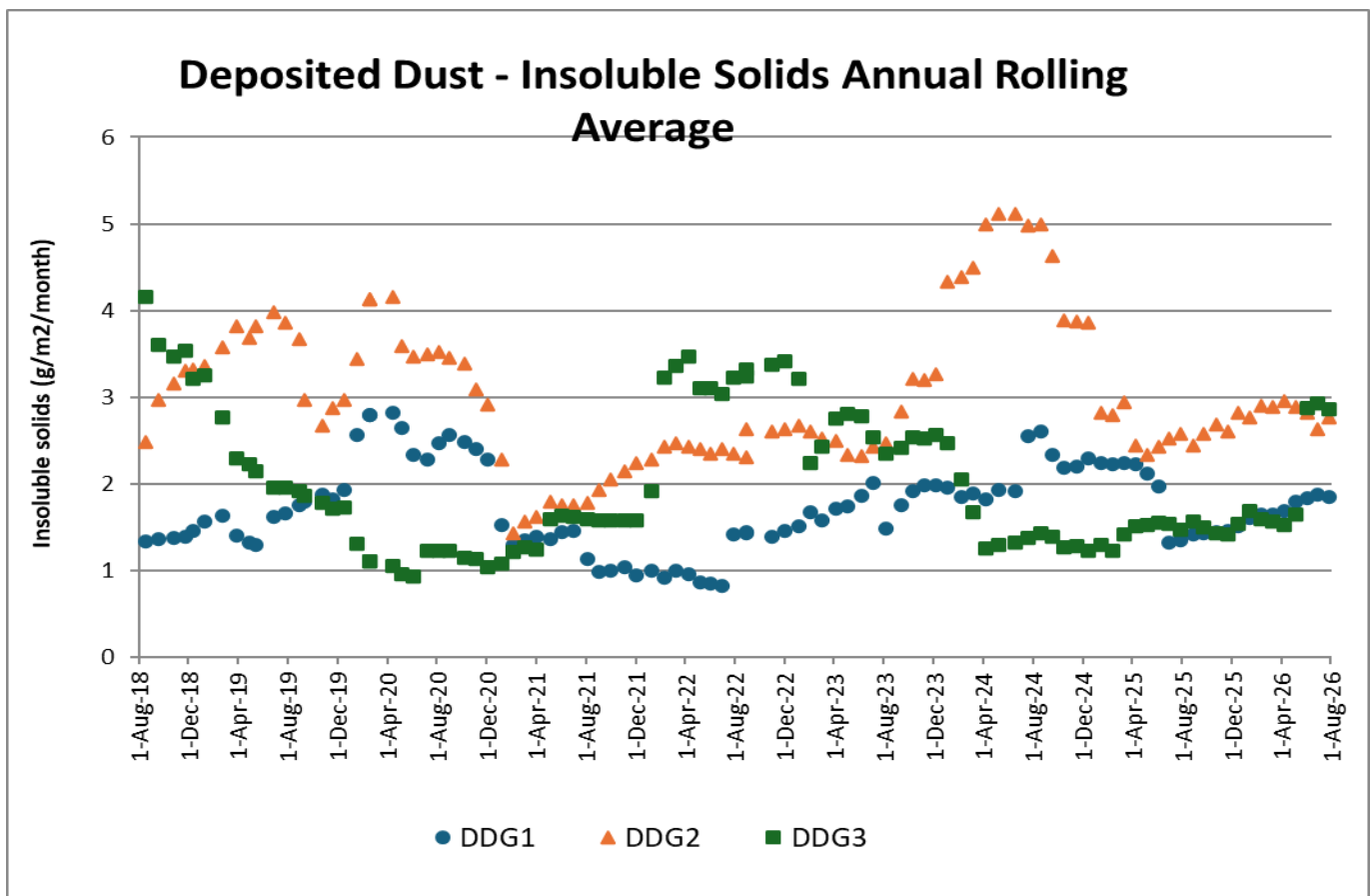
Figure 2 – Monthly Dust Annual Rolling Average – Insoluble Solids
