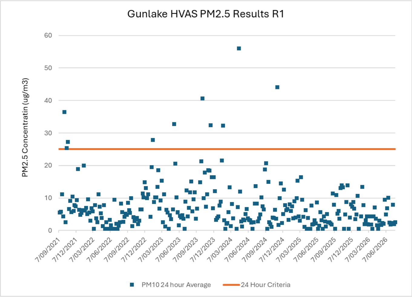
Figure 5 – HVAS PM2.5 Monitoring Results
