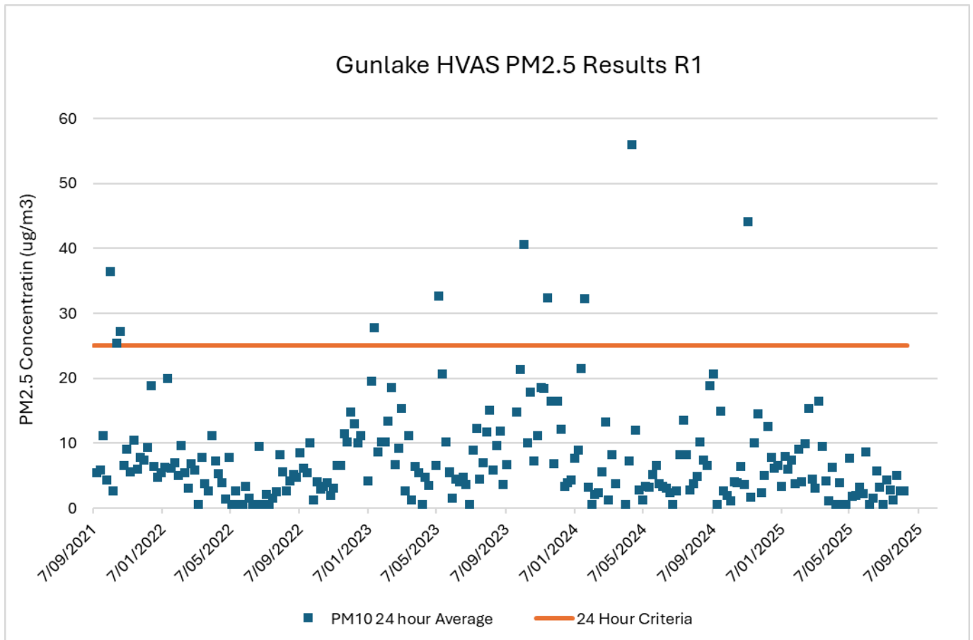
Figure 5 – HVAS PM2.5 Monitoring Results
